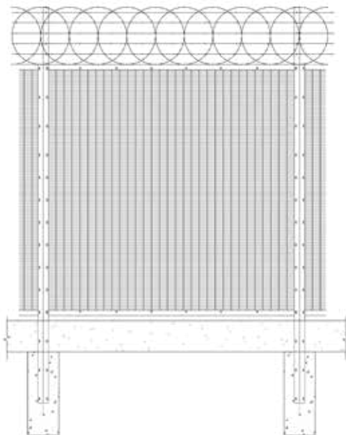
3000MM HIGH ASSEMBLY INCLUDING RAZOR TAPE TOPPING*
