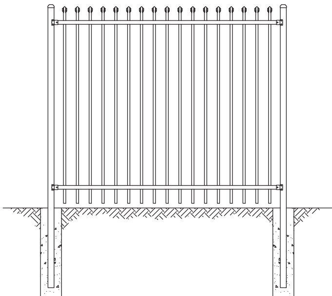
2100mm HIGH PANEL & POST ASSEMBLY*
